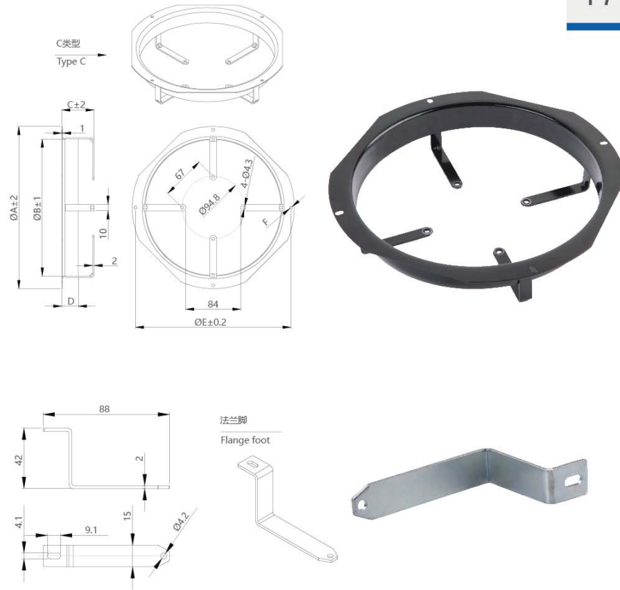
规格尺寸 Specification size
