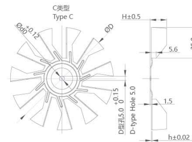
风叶规格尺寸 Fan specification and dimension
