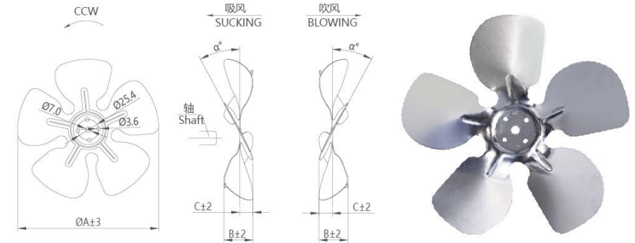
风叶规格尺寸 Fan specification and dimension
