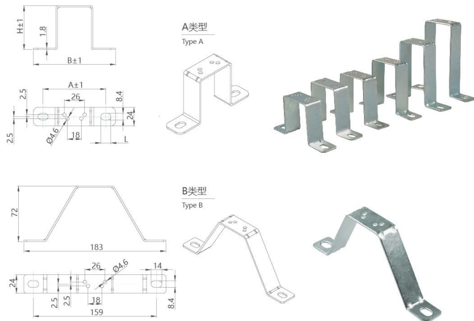
A类型规格尺寸 Type A specification size
